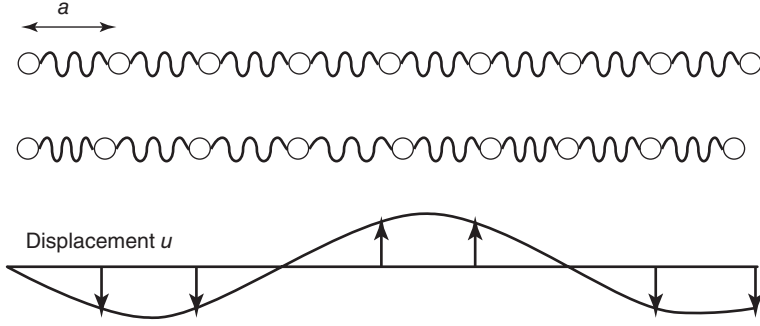
Figure 2.1 A one-dimensional linear chain. The atoms are shown in their equally spaced equilibrium conditions in the top row and with a periodic distortion below. The bottom figure plots the displacements u_n as arrows, and the curve shows how this is a sine wave of period 6a in this case. (Reproduced with permission of PB Littlewood and Premi Chandra.)
