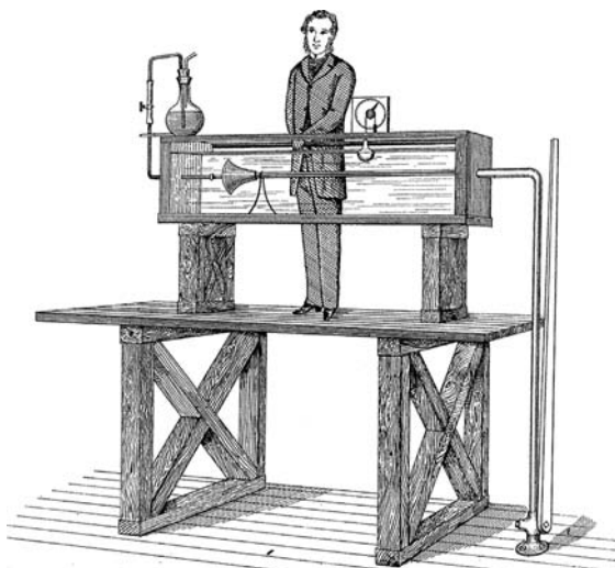
Figure 1.3 The original apparatus used by Osborne Reynolds to study the motion of water [7]. The apparatus consisted of a tank filled with
