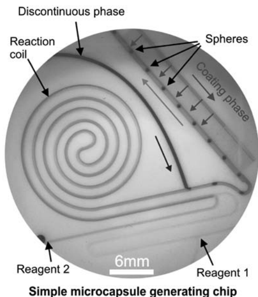
Figure 1.1 Detailed example of a simple duct-based microreactor fabricated from polytetrafluoroethylene (with perfluoralkoxy capping layer). Reagents 1 and 2 interact by diffusive mixing within the reaction coil. The reaction product becomes the continuous phase for an immiscible discontinuous phase,
