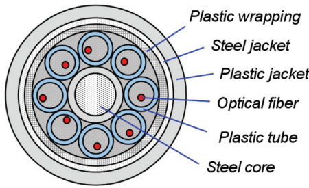
Figure 2.3 Schematic cross-section of a typical fiber cable.
