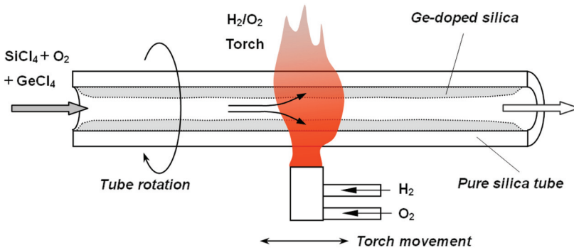
Figure 2.2 Schematic diagram of MCVD process for silica fiber preform.
