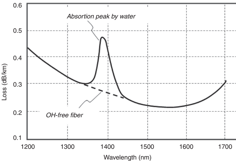
Figure 2.4 Typical loss spectrum of silica fibers. (Reprinted with permission from reference [20].)
