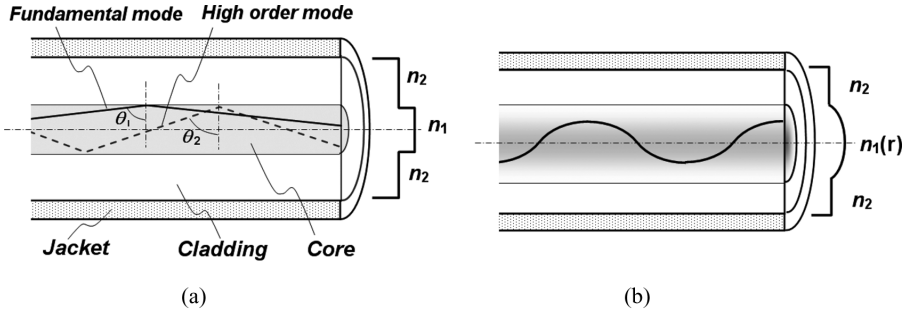
Figure 2.1 Schematic illustration of optical fibers: (a) step-index fiber and (b) gradient index fiber.
