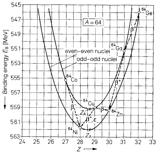
Figure 2.5. Binding energy and transmutation of nuclides with even mass numbers.
