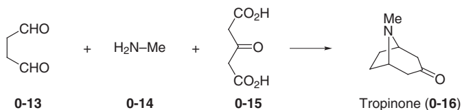
Scheme 0.5. Domino process for the synthesis of tropinone ( 0-16 ).
