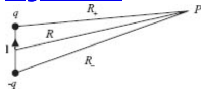
Figure 1.1 Induced dipole
