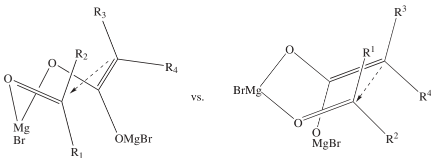
TS A: chairlike transition structure
