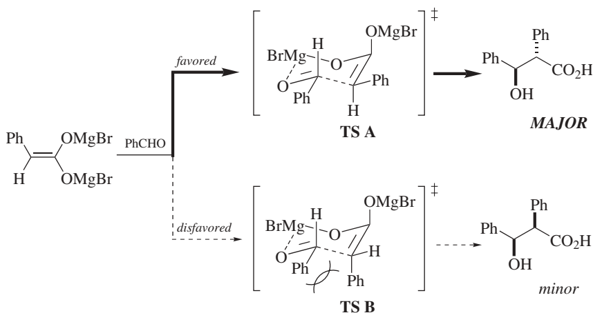
Scheme III
