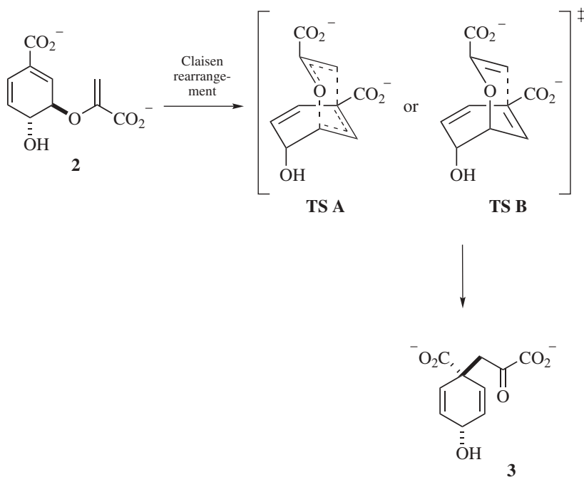
Scheme IV
