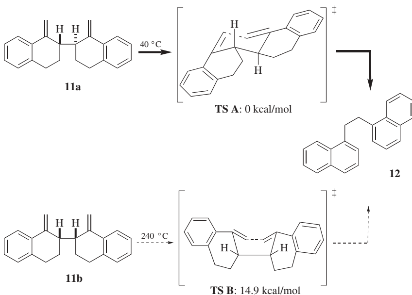
Scheme 1.XI
