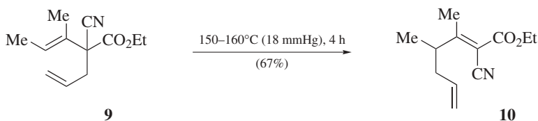
Scheme 1.X
