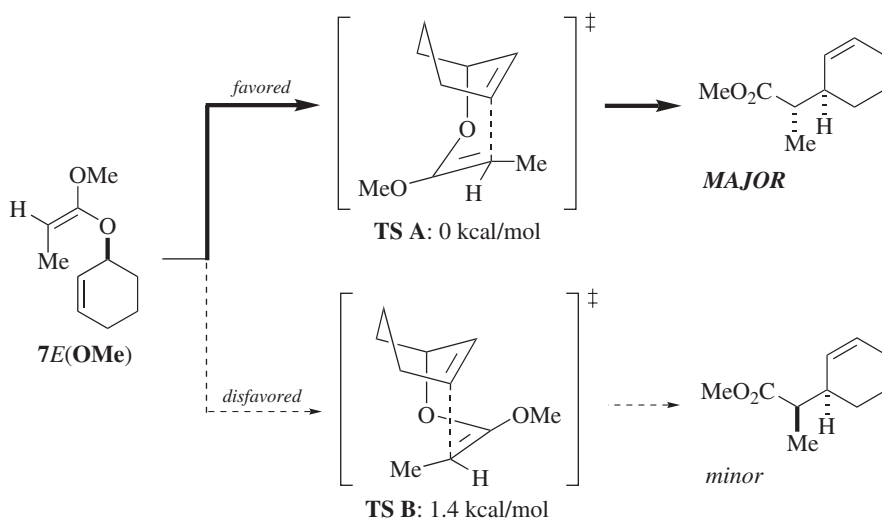
Scheme 1.IX
