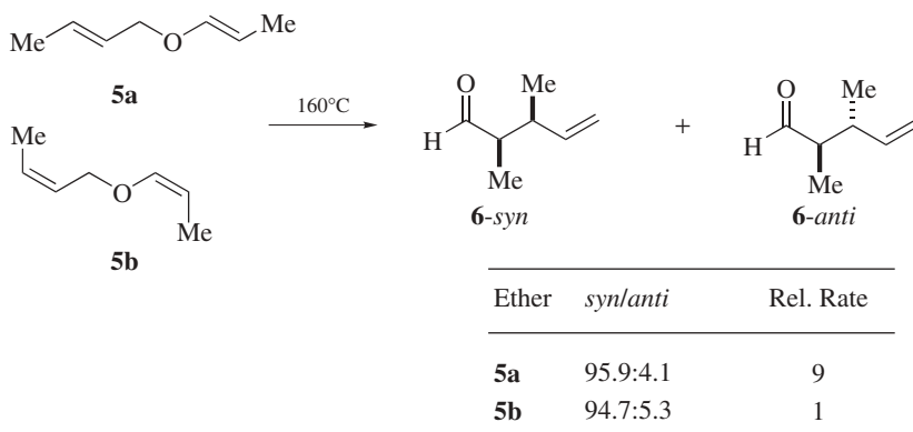
Scheme 1.V
