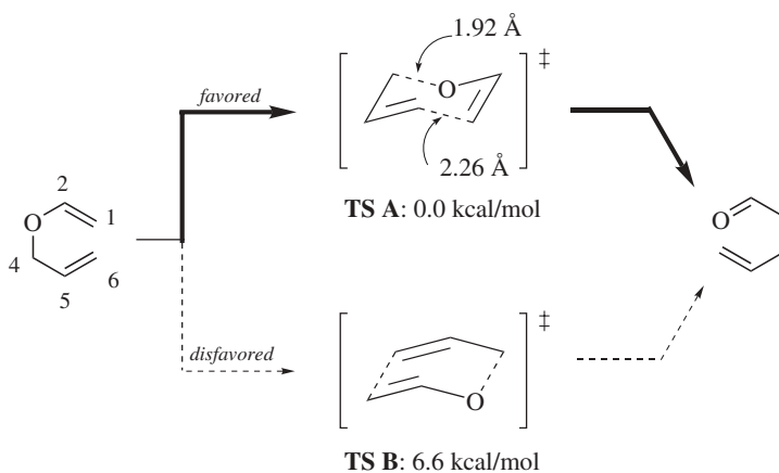
Scheme 1.IV
