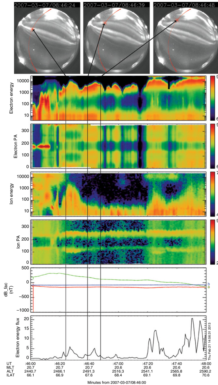
Figure 1.3 Example of inverted-V acceleration and the resulting aurora, reprinted from Colpitts et al. [2013] . Top panels: KIAN images for 08:46:24, 08:46:39, and 08:46:48 UT with mapped FAST trajectory (red line) and location (red star) overplotted. Lower panels: FAST data from 08:46–08:48 UT, with black vertical lines representing the times of the KI–south (red line), AN images; magnetometer panel (second from bottom) shows perturbations in the north east–west (green) and vertical (blue) directions.
