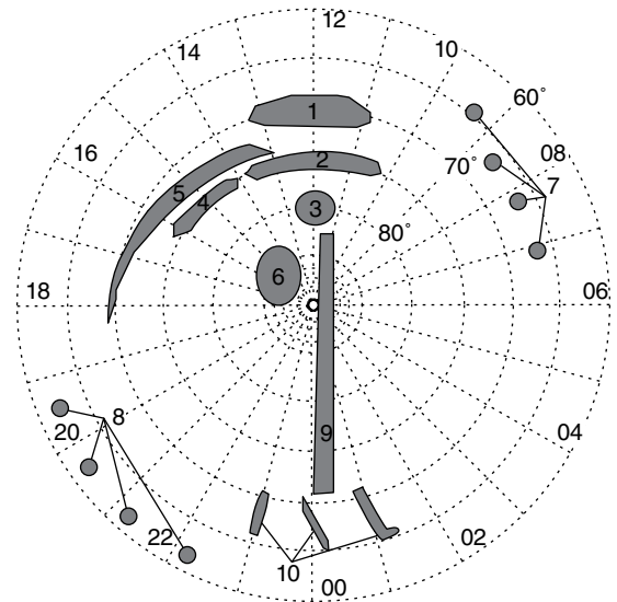
Figure 1.9 Anomalous aurora, from Frey [2007].
