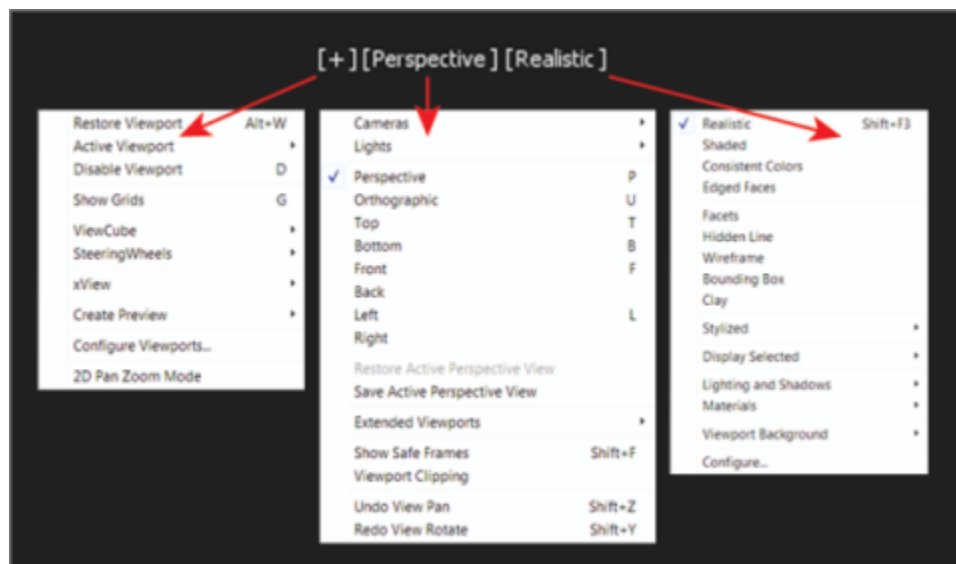
FIGURE 1.3 Viewport label menu showing the General Viewport, Point-of-View, and Shading Viewport menus.
