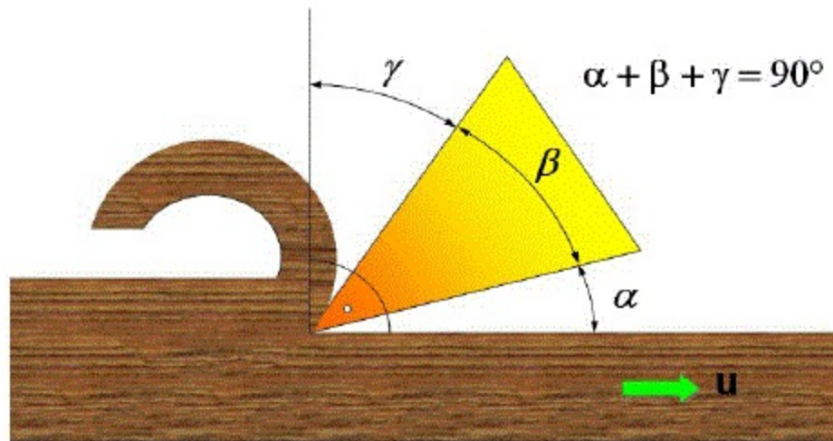
Figure 1.4. Simplified cutting process model
