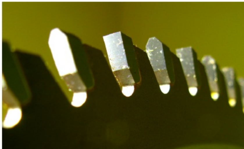
Figure 1.11. Saw blade with the tooth shape optimized for cutting laminated panels
