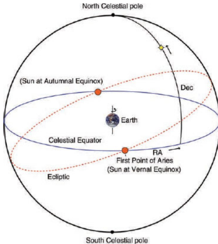
Figure 1.6 The celestial sphere.
