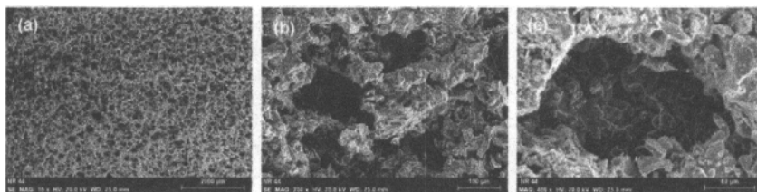
Figure 1. SEM micrographs of porous structure of 45S5 scaffolds sintered at 975^\circ \text{C} at various magnifications: (a) 15x, (b) 200x, and (c) 400x.
