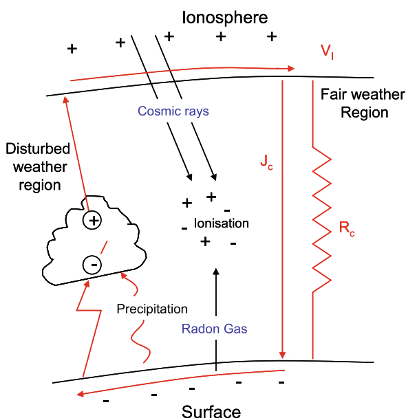
Fig. 2 Simplified “electrical engineering” model of the global circuit, illustrating charge generation in disturbed weather regions, conduction through the ionosphere (upper layer) and surface (lower layer), and discharge through the finite conductivity of fair weather regions. In fair weather regions, the ionospheric potential V_i , conduction current density J_c and unit area columnar resistance R_c are related by Ohm’s Law
