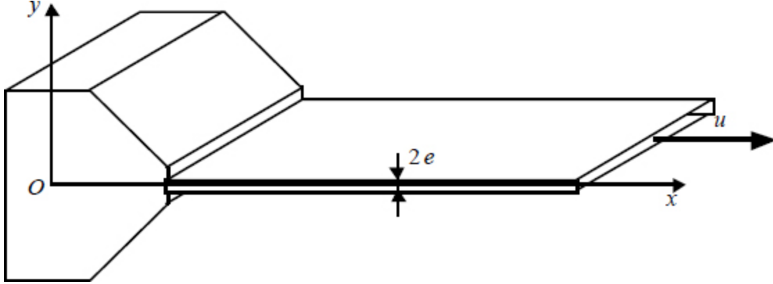
Figure 1.4. Cooling of a film exiting the die
