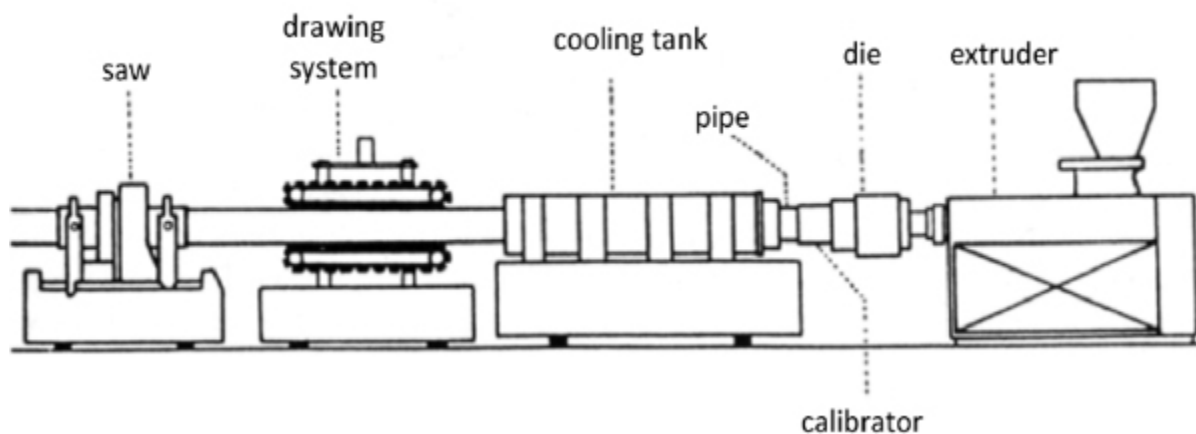
Figure I.2. Example of a pipe extrusion line
