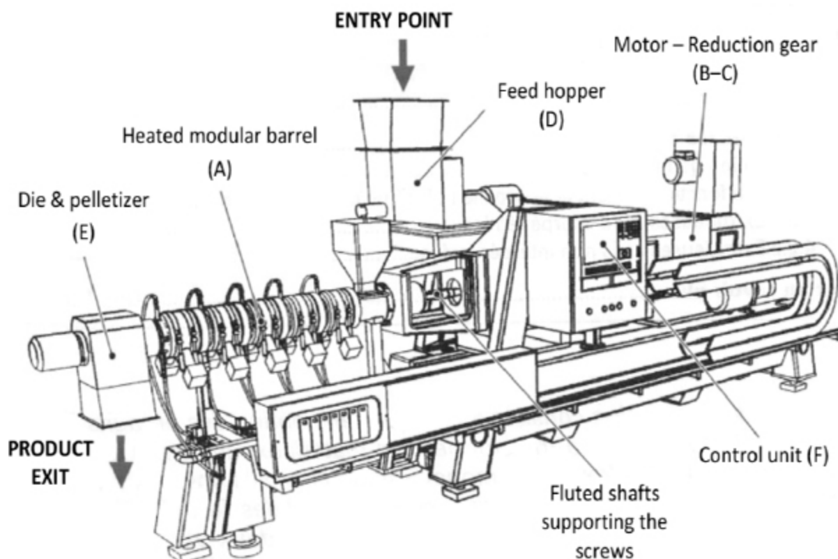
Figure I.1. Diagram of a co-rotating twin screw extruder (Source: Clextral)
