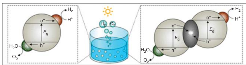
Figure 1.6 Representation of single semiconductor (left) and double-semiconductor Z-scheme (right) designs for overall water splitting photocatalysts incorporating dedicated co-catalysts for \text{H}_2 and \text{O}_2 evolution. Reproduced with permission from Ref. [22]; Creative Commons 2022 American Chemical Society.
