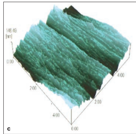
Fig 1-4 (a) The original Brånemark machined-surface implant. (b and c) Machined-surface topography.
