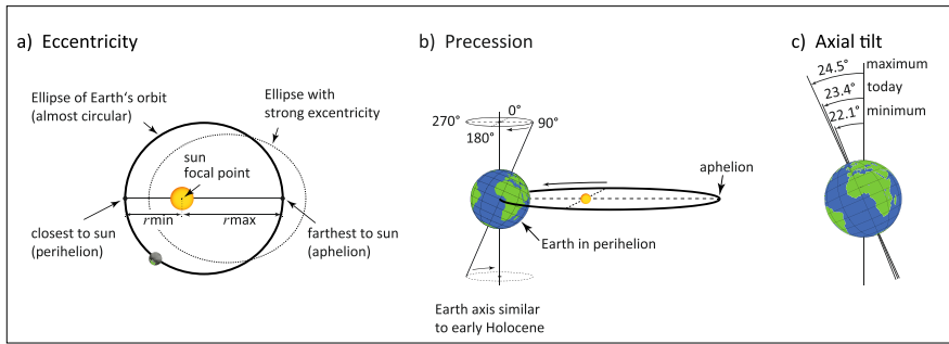
Fig. 1.8. Based on three quasi-periodic mechanisms, the position and orientation of the Earth relative to the Sun's changes causes variations of the solar insolation, called Milanković forcing. a) Change of the elliptical path of the Earth around the Sun. b) Wobbling of the Earth's axis, called precession. c) Change of the obliquity (tilt) of the Earth's axis.
