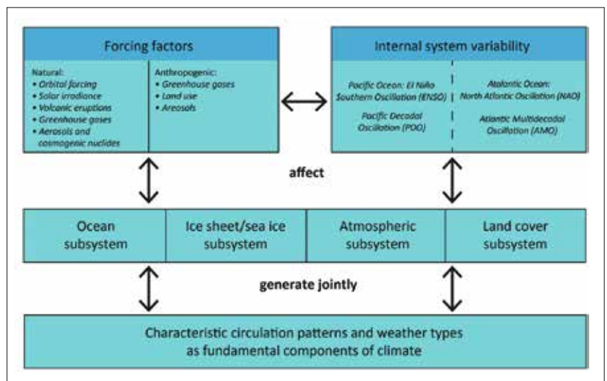
Fig. 1.6. Pattern of interaction showing the key factors and processes influencing weather and climate.
