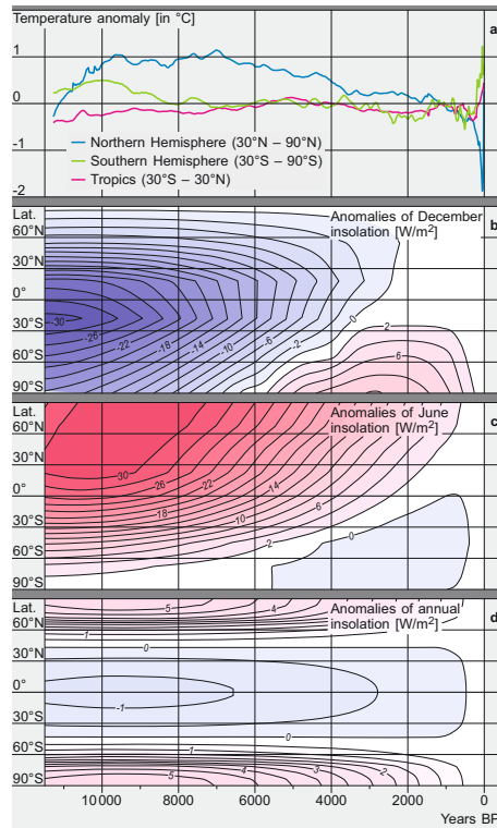
Fig. 1.9. a) Reconstructed Holocene temperature time series for three regions of the globe (°C). b) Anomalies of the average solar insolation at the Earth's surface during December (W/m 2 ). c) Same as b, but for June. d) Annual average solar insolation.
