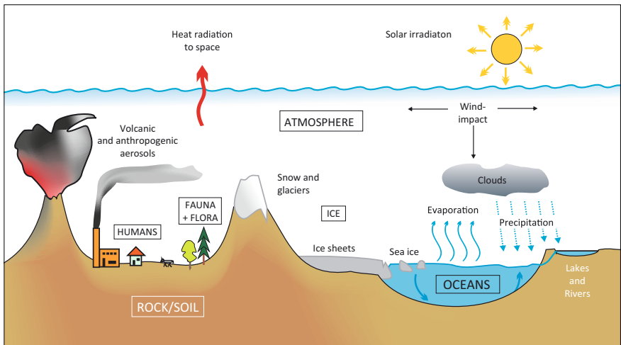
Fig. 1.5. Climate system of the Earth. The subsystems are represented in rectangles. Important processes or phenomena are also noted.
