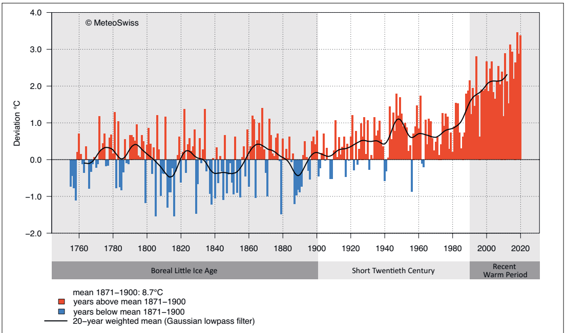
Fig. 1.1. Anomalies of annual mean temperatures in Basel/Binningen, Switzerland, from 1755 to 2020 (with respect to the 1871–1900 mean; source: Bundesamt für Meteorologie und Klimatologie MeteoSwiss). https://www.meteoswiss.admin.ch/home/climate/climate-change-in-switzerland.html ; accessed 3 January 2020.
