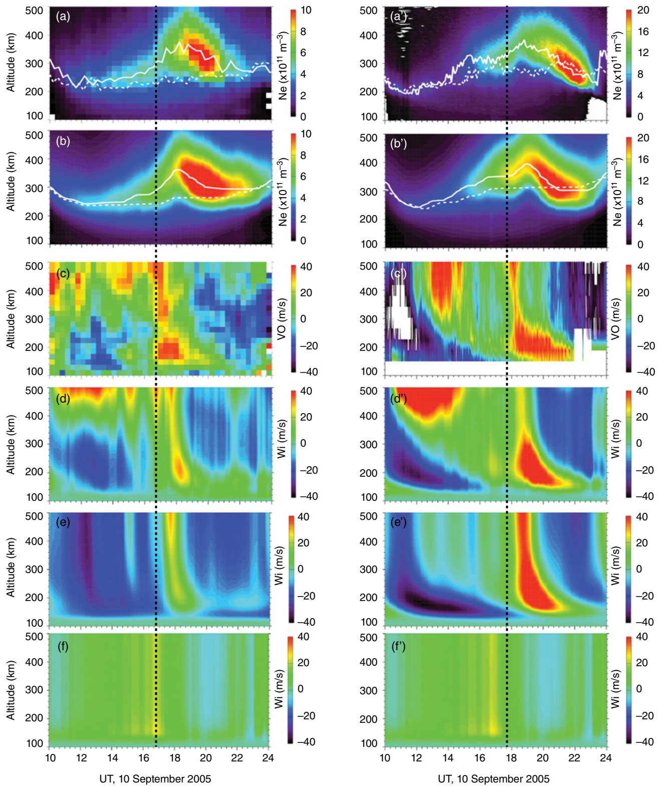
Figure 1.3 UT versus altitude profiles of row (a) and (a') measured electron density; row (b) and (b') simulated electron density; row (c) and (c') measured vertical ion drift; row (d) and (d') simulated vertical ion drift; row (e) and (e') simulated vertical ion drift due to neutral wind; and row (f) and (f') the simulated vertical ion drift component due to electric field. The solid white lines show the row (a) and (a') observed and row (b) and (b') simulated h_m F_2 on the storm day of 10 September, and the dashed white lines indicate the corresponding h_m F_2 on the quiet day of 8 September. The vertical dashed lines mark the onset of upward lift of electron density peak height over (left column) Millstone Hill and (right column) Arecibo. Source: Lu et al. (2008), Figure 2, p. A08304(3). Reproduced with permission of the American Geophysical Union.
