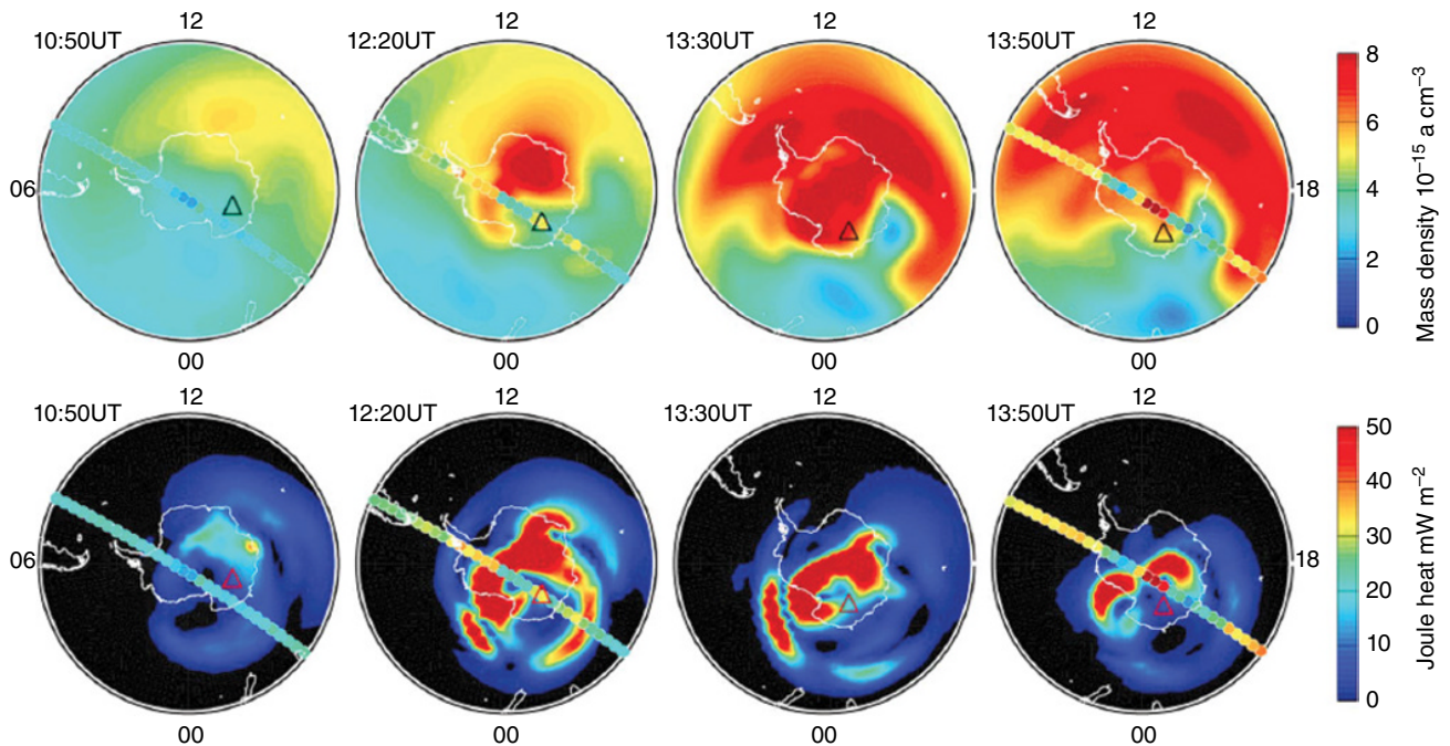
Figure 1.4 Maps of (top row) neutral mass density at 380 km and (bottom row) height-integrated Joule heating over the southern hemisphere. The small colored dots indicate the CHAMP trajectory, with the color of each dot corresponding to the mass density value measured by CHAMP using the color scale from the top row. The outer circle corresponds to 40^\circ S , and the triangle in each map indicates the magnetic south pole. Source: G. Lu et al., 2016, Figure 4, p. 7115. Reproduced with permission of the American Geophysical Union.
