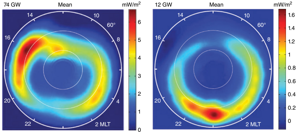
Figure 1.1 (Left) Average of the 30 sample distributions, covering all seasons and geophysical conditions, used for constructing the Poynting flux model. The hemispherically integrated flux is 74 GW. (Right) Average of the 30 sample distributions, covering all seasons and geophysical conditions, used for constructing the kinetic energy flux model. The hemispherically integrated flux is 12 GW. Note the different color scales on the left and right. Source: Cosgrove et al. (2014), adapted from (left) Figure 2, p. 418, and (right) Figure 14, p. 427. Reproduced with permission of the American Geophysical Union.
