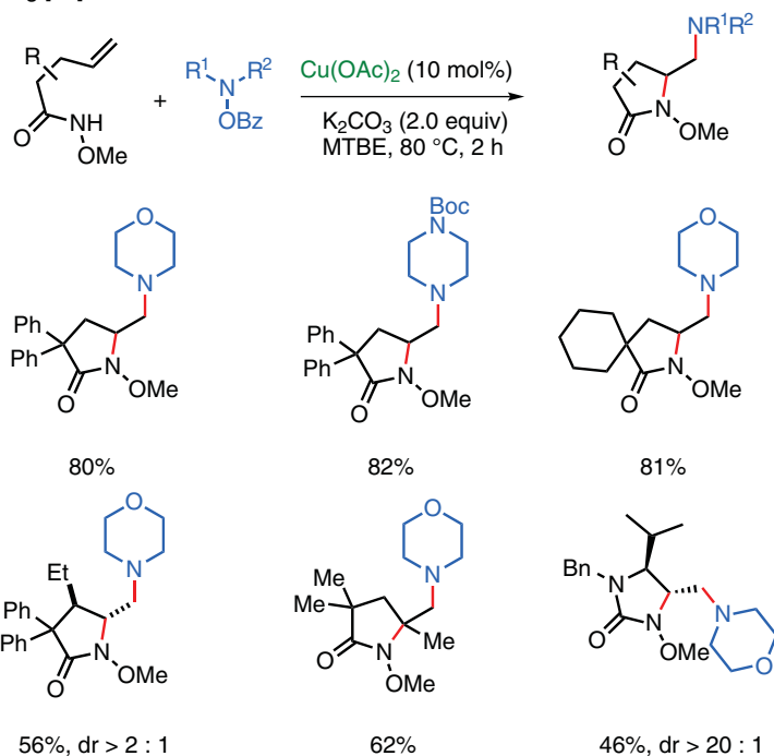
Scheme 1.18 Cu-catalyzed electrophilic diamination. Source: Modified from Shen and Wang [25].
