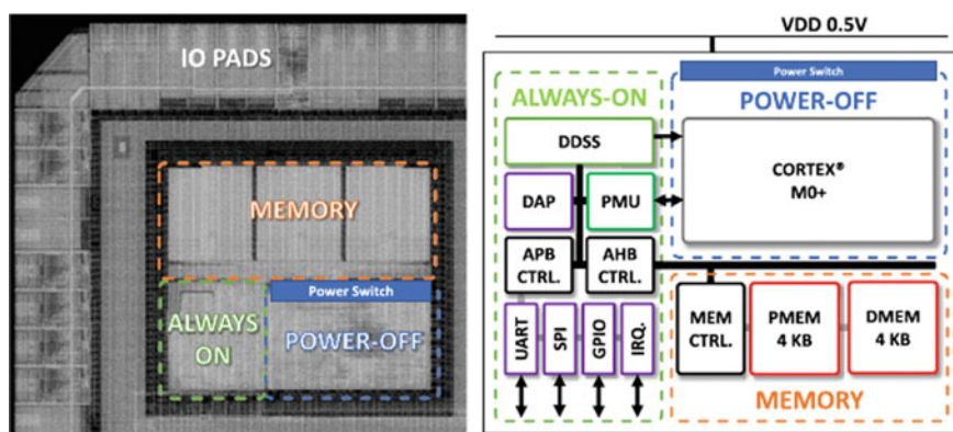
Fig. 3 28nm FD-SOI SoC implementation and corresponding block diagram. Core area is 0.073 \text{ mm}^2 [35] ©[2018] IEEE
