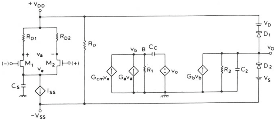
Fig. 4 The macromodel for integrated all-MOS operational amplifiers [57] ©[1983] IEEE
