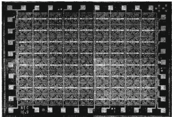
Fig. 1 The photograph of an 144-bit ( 16 \text{ word} \times 9 \text{ bit} ) n -channel MOS-LSI memory. The chip area is 4.3 \times 3.0 \text{ mm} [55] ©[1969] IEEE
