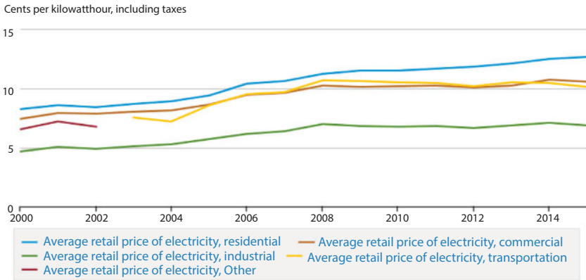
Figure 1.2 Average retail prices of electricity [5].
